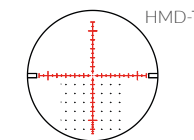
Subtensions of HMD-T reticle see page 30.
