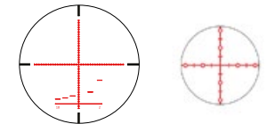
SUBTENSIONS: SKELETON HMD (HALF MIL DOT)
